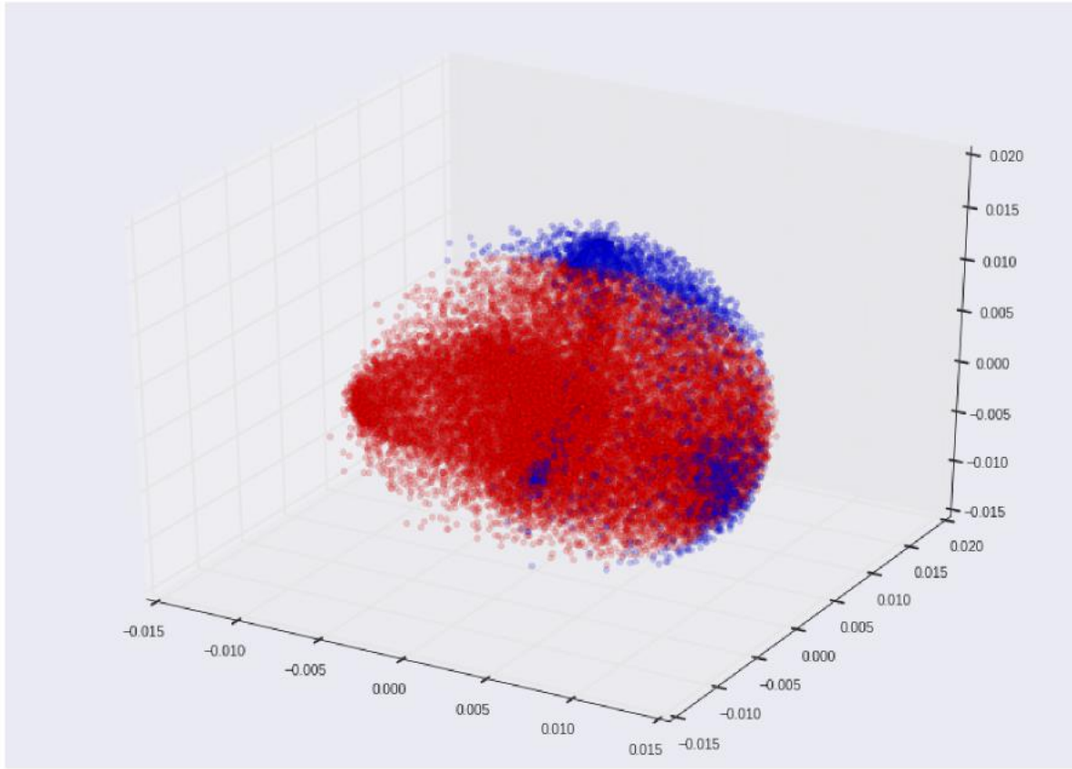
Supplemental Figure S6: Loadings for first three principal components of each gene. Genes in blue represent the 2,500 genes with the greatest sum magnitude of loadings for PC1, PC2, and PC3.
